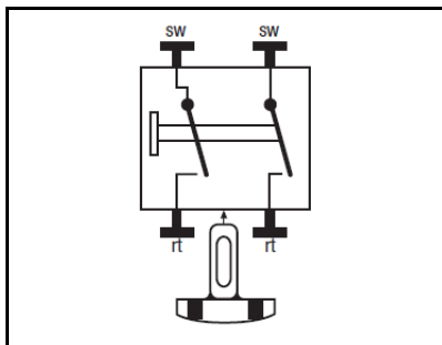
Contact assignments
